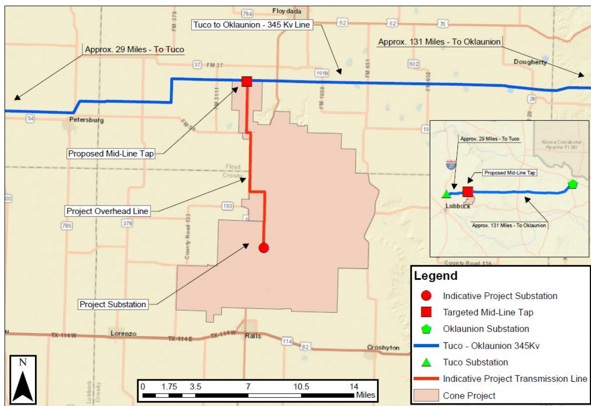
Figure 1 – New Whirlwind Substation Location
